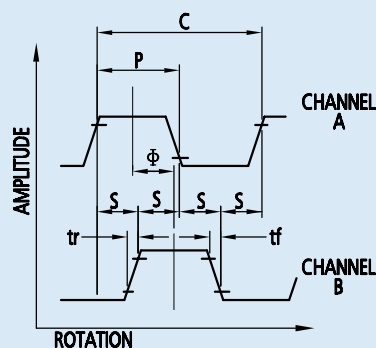
OUTPUT SIGNALS with clockwise rotation as seen from the shaft end exceptions indicated by note 3
